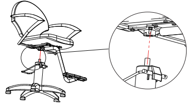
2. Connect the backrest to the gas lift with a dowel, then insert the cotter pin.
