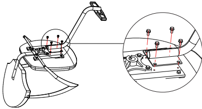
1. Use 4 pcs bolts (M8*20) to fix the seat inclination
